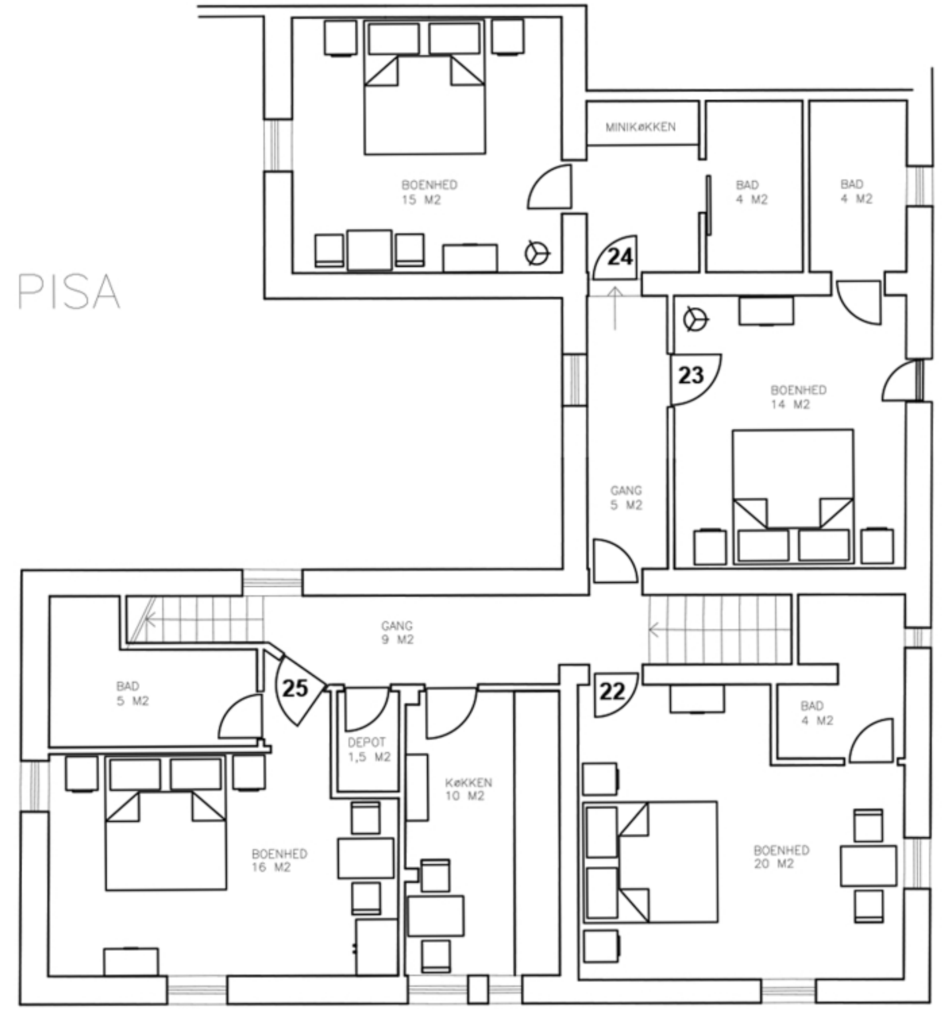
FIRST FLOOR
